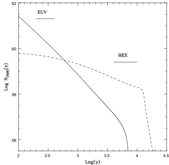
Figure 3: Plot of the energy distribution of the relativistic electron populations in the Coma cluster. The dashed line represents the main electron population, integrated over the cluster volume, injected during the first phase and reaccelerated during the second phase . The solid line refers to the additional electron population injected by the radio galaxy NGC 4869. The typical energies of the electrons emitting via IC in the hard X-ray band (HEX) and in the EUV band are also indicated.
